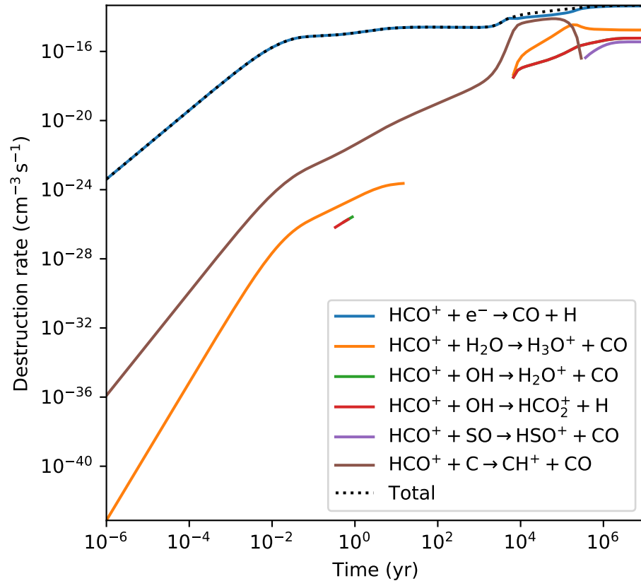
Main HCO + destruction routes
