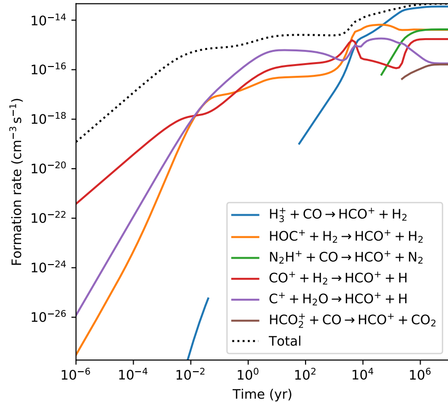
Main HCO + formation routes
